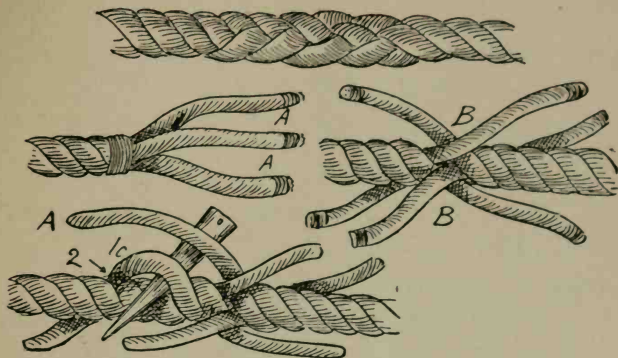
FIG. 106.—Short splice.
